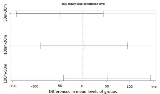
Figure 5. Post-hoc Tukey HSD test results of Conductivity (µS/cm) in the water column between riparian zone width categories.
