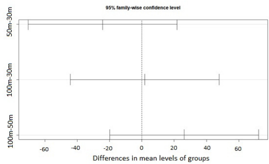
Figure 4. Post-hoc Tukey HSD test results of Total Dissolved Solids (mg/l) in the water column between riparian zone width categories.
