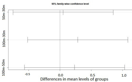
Figure 2. Post-hoc Tukey HSD test results of Organic Matter percentage in the sediment between riparian zone width categories.
