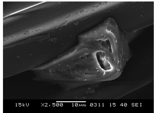
Figure 4 SEM-Rusch Flat Filter, S. aureus 2500× magnification, after bacterial infusion.
