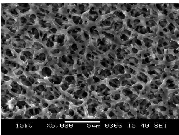
Figure 2 SEM-Portex Flat Filter; Granular structure 5000× magnification, before bacterial infusion.
