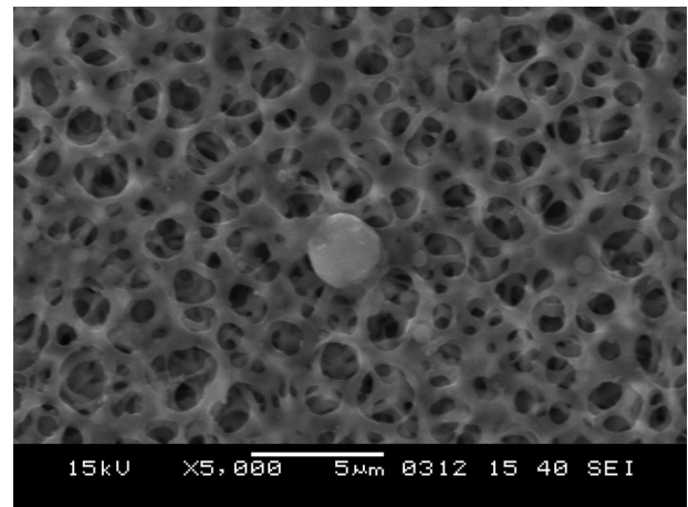
Figure 3 SEM-Portex Flat Filter, Staphylococcus aureus 5000× magnification, after bacterial infusion.
